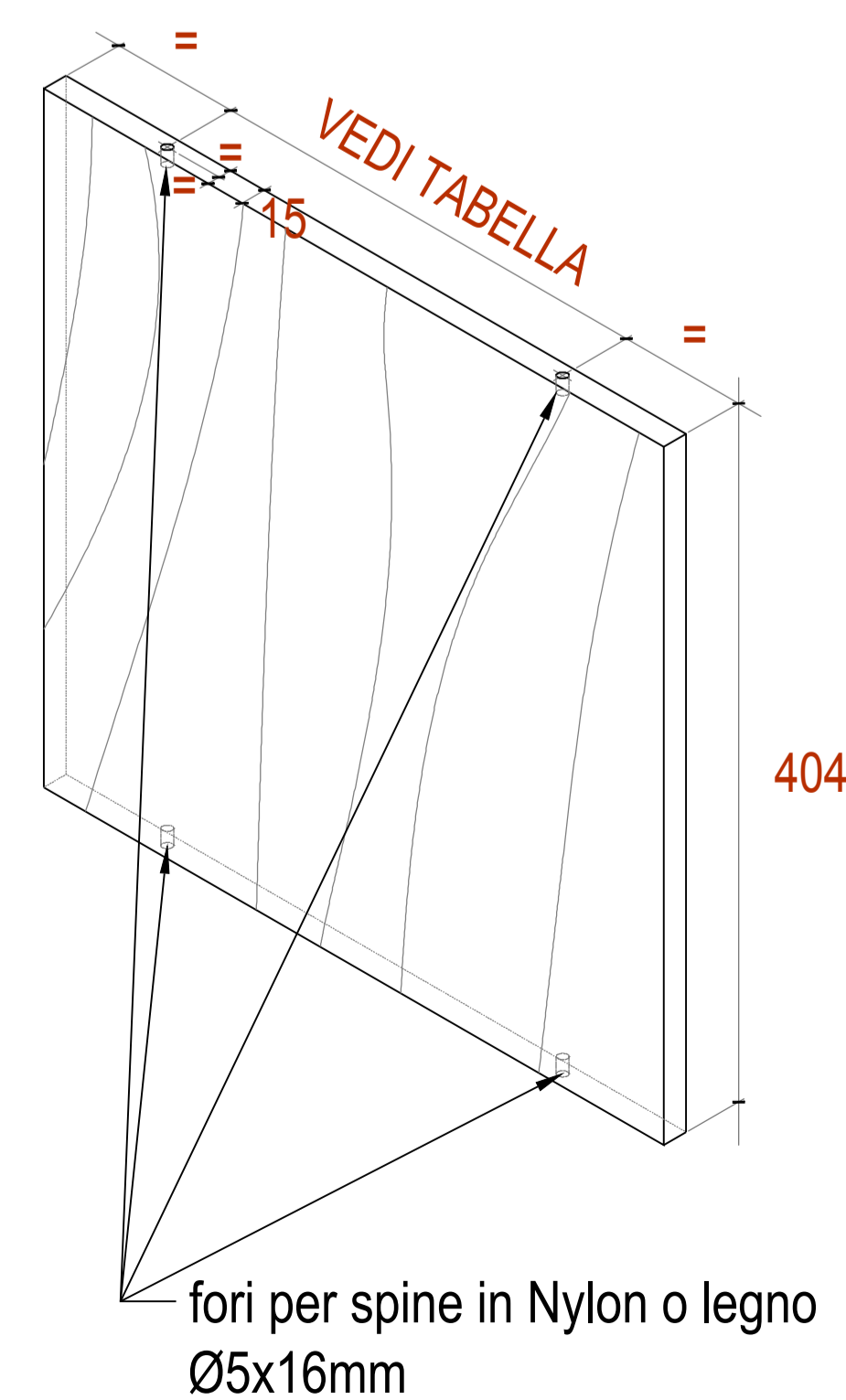
SETTI IN MARMO - 1:4
